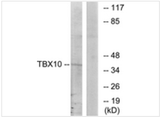
Western blot Western blot analysis of extracts from HT-29 cells, using TBX10 Antibody. The lane on the right is treated with the synthesized peptide
