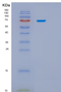
Figure 1. SDS-PAGE
