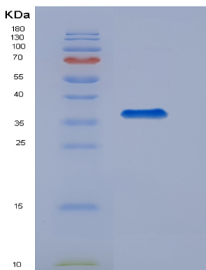
Figure 2. SDS-PAGE
